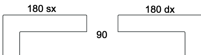
art. 10 - schienale cm. 180 x 90dx o sx art. 10 - backrest cm. 180 x 90 L/R
