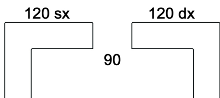
art. 9 – schienale cm. 120 x 90 dx o sx art. 9 - backrest cm. 120 x 90 L/R
